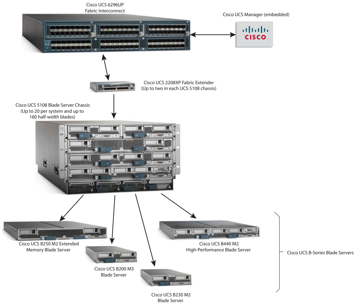
Figure 7 System Diagram
