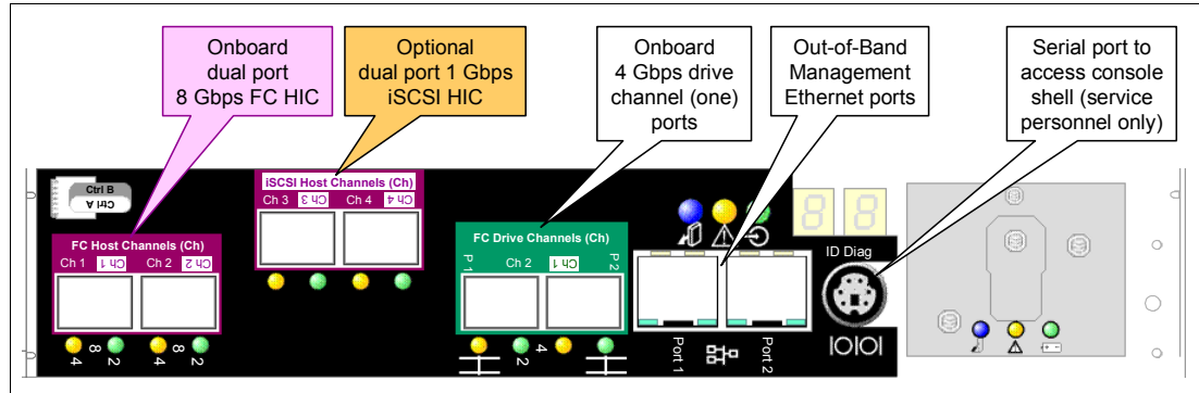
Figure 7 DS3950 controller with iSCSI host ports
