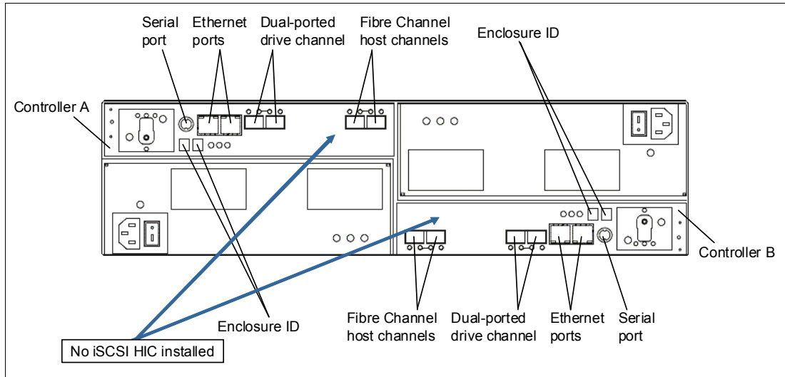
Figure 3 DS3950 rear view: four FC ports (model 94H)
