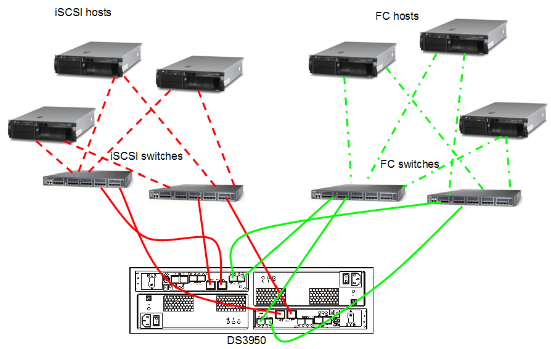
Figure 10 DS3950 mixed host connection layout
