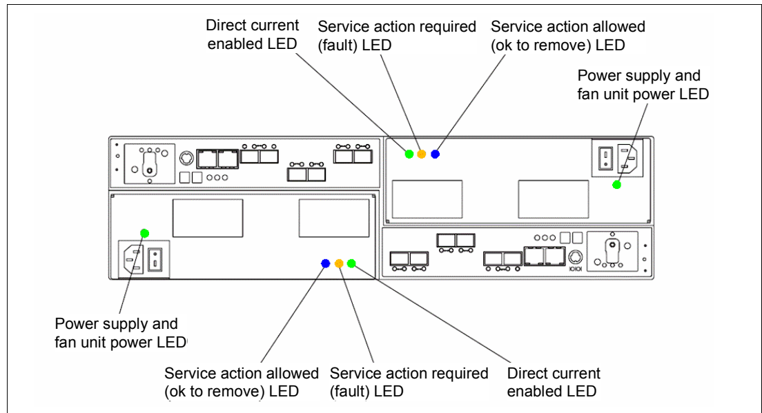
Figure 6 DS3950 power supply and fan unit LEDs
