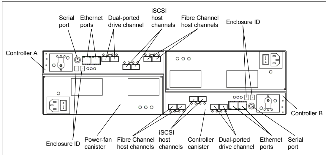
Figure 9 DS3950: All connectors
