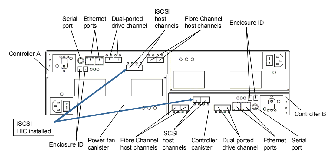
Figure 4 DS3950 rear view: four FC and four iSCSI ports (model 98H)
