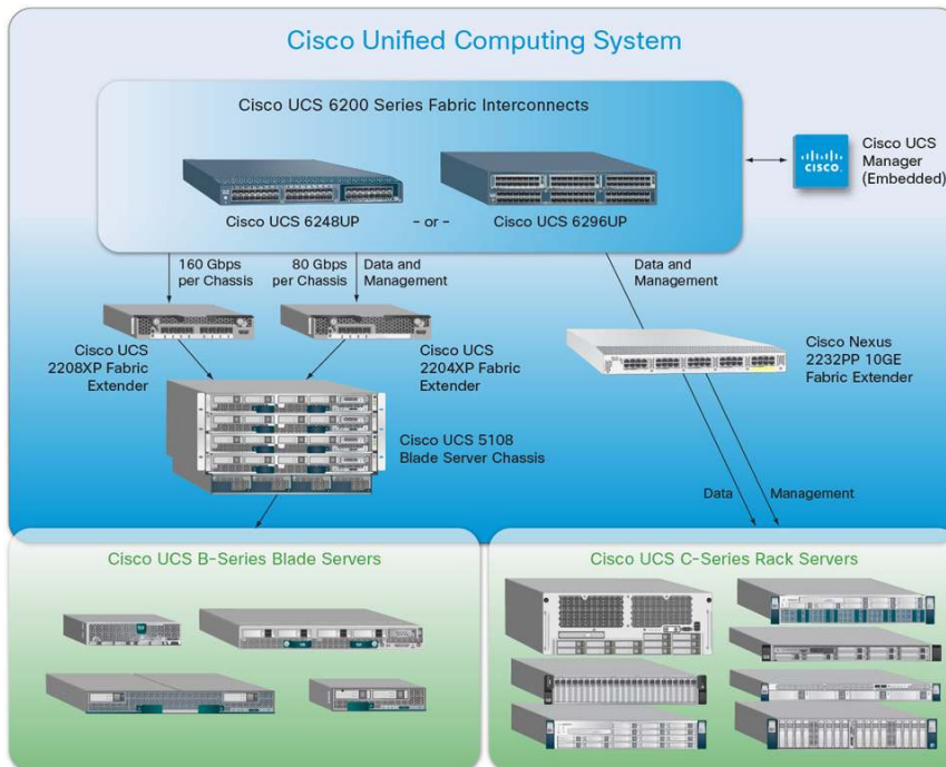
Figure 2. Cisco UCS Components
