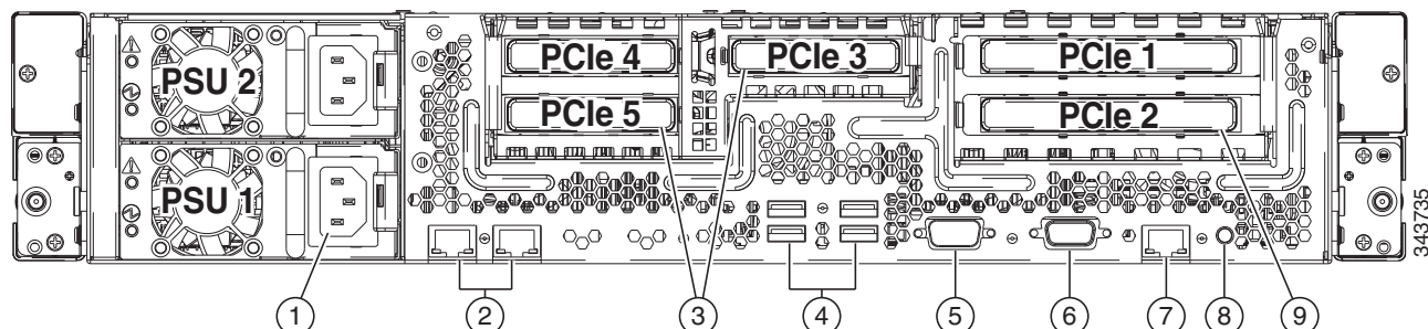
Figure 2 Chassis Rear View
