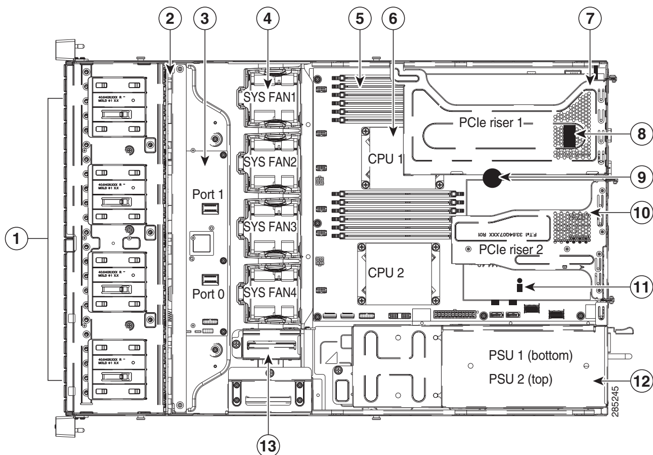
Figure 5 C24 M3 LFF With Top Cover Off
