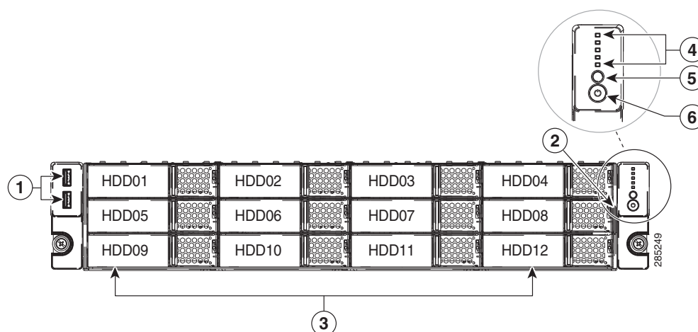
Figure 1 Chassis Front View
